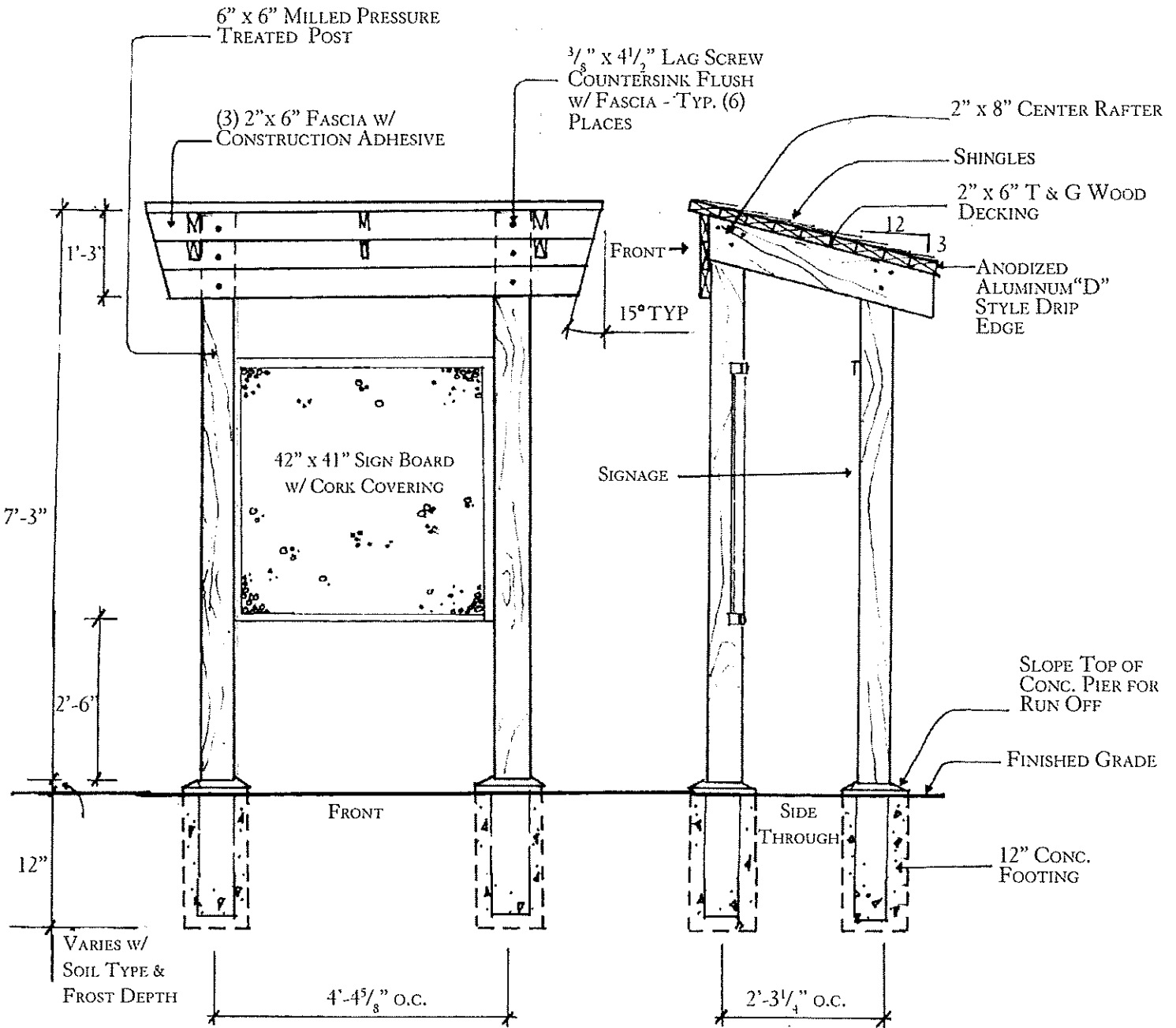
1 PLAN & SECTION OF WOODEN KIOSK L1.8 NTS
